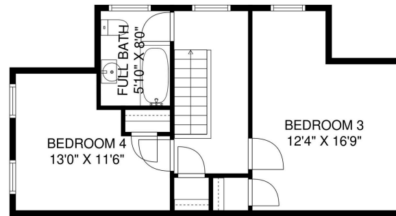
THIRD FLOOR
