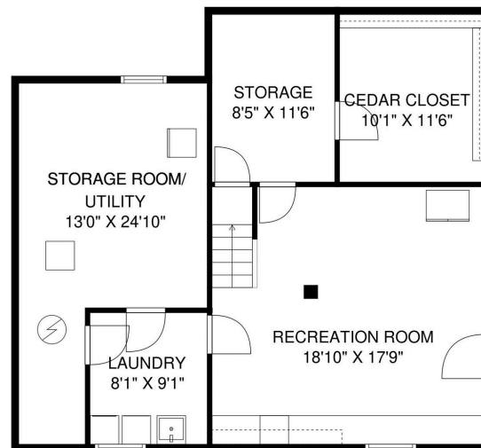
LOWER LEVEL
